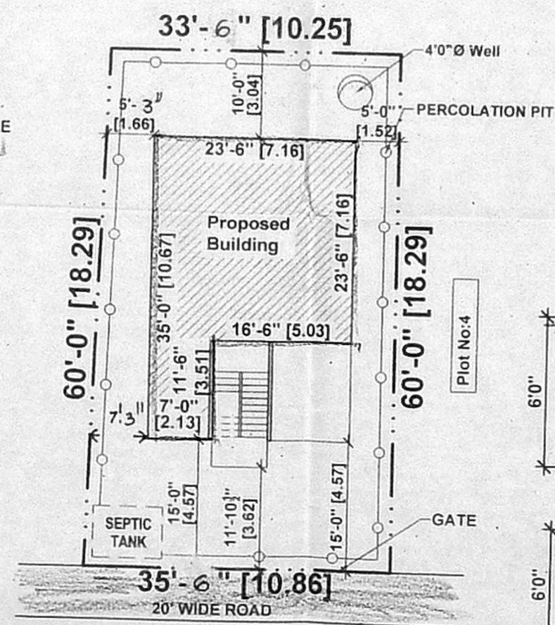
Site Plan
