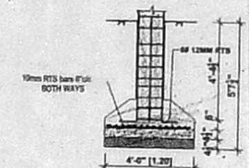
DETAILS OF FOUNDATION SCALE 1:50 (1"=40')
